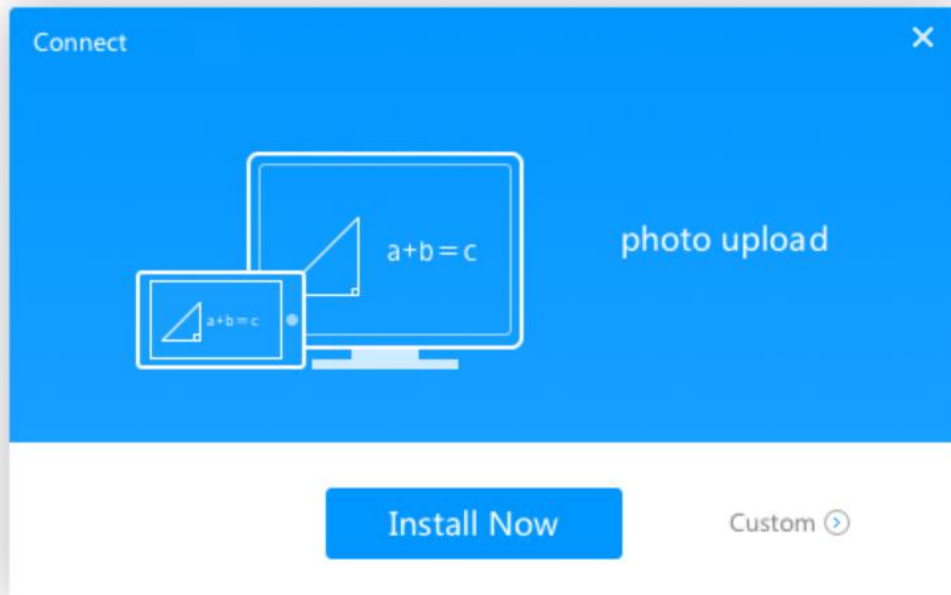
Figure 2-2-1 Installation interface
