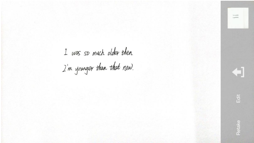
Figure 3-2-2-2 camera interface
