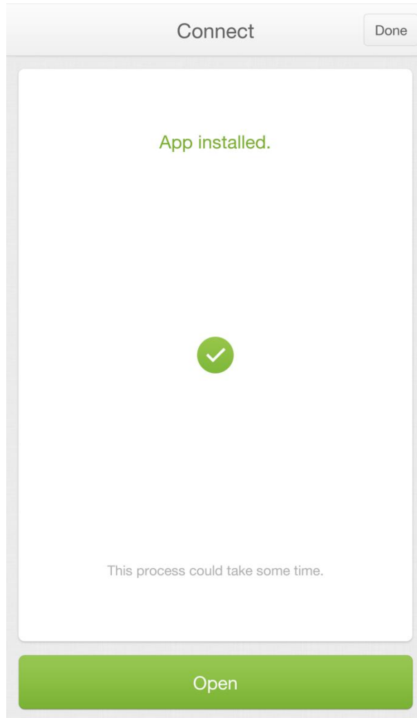
Figure 2-3-2 Installation completion
