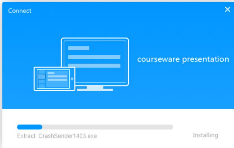
Figure 2-2-2 Installation progress
