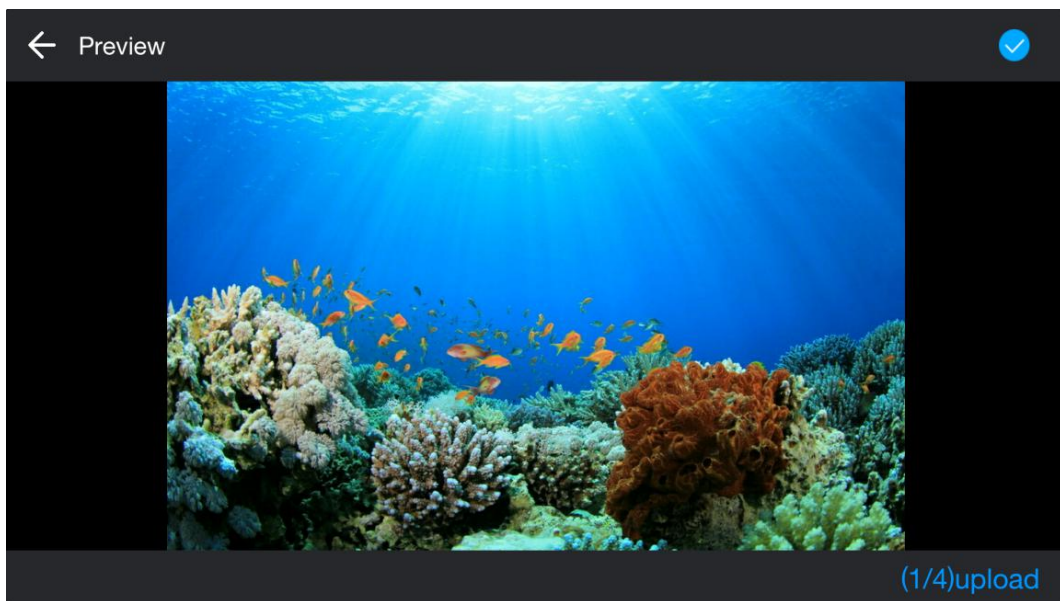
Figure 3-2-5-2 Picture preview
