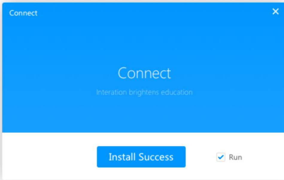
Figure 2-2-4 Installation completion
