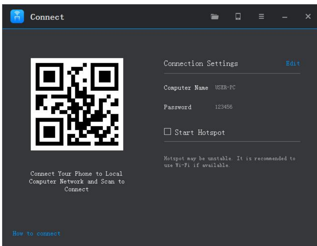
Figure 3-1-1 PC
