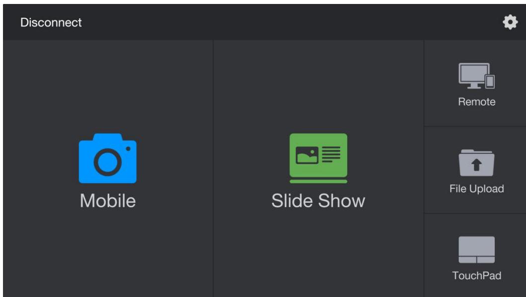
Figure 3-2-1-5 Main interface
