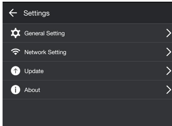
Figure 3-2-7-1 Settings interface
