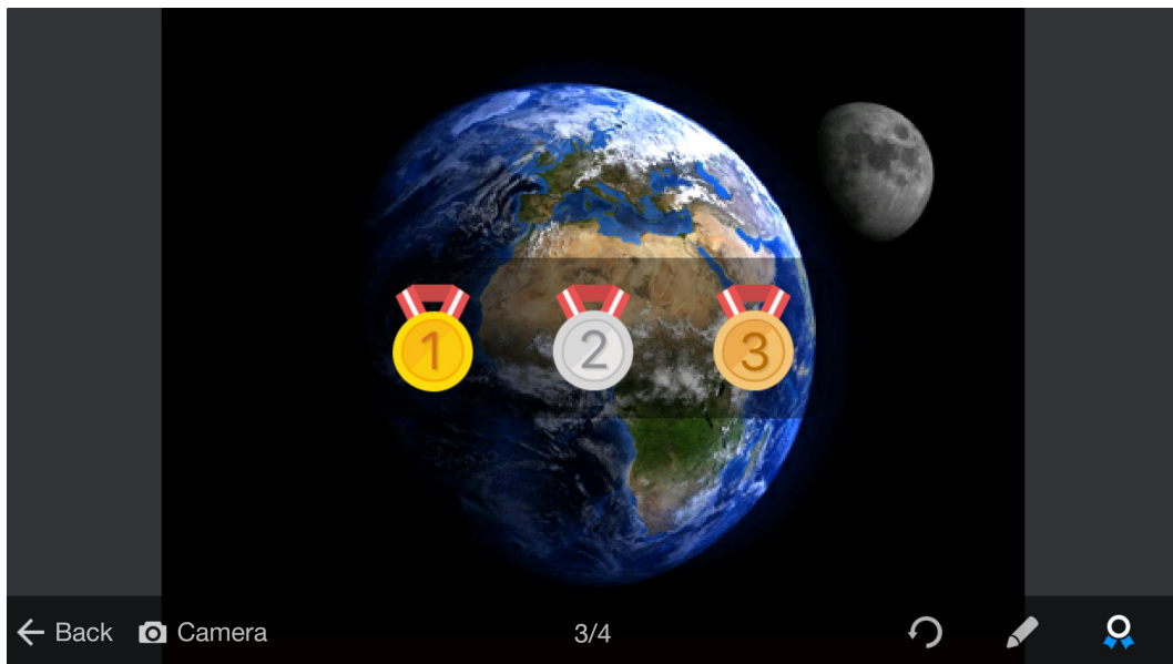
Figure 3-2-2-8 Medal mode
