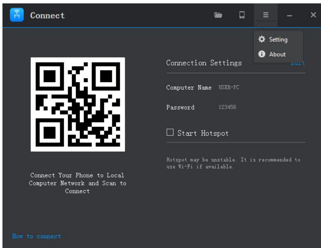
Figure 3-1-2 More interface
