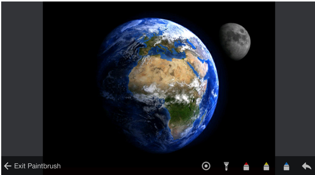
Figure 3-2-2-7 Paintbrush
