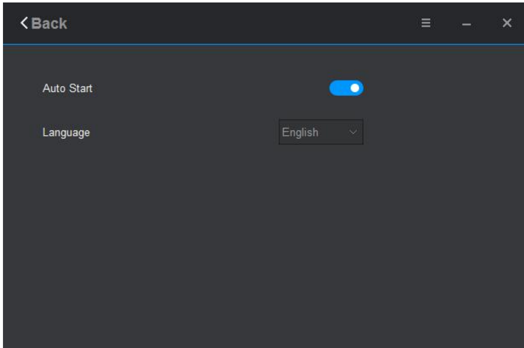
Figure 3-1-3 setting interface
