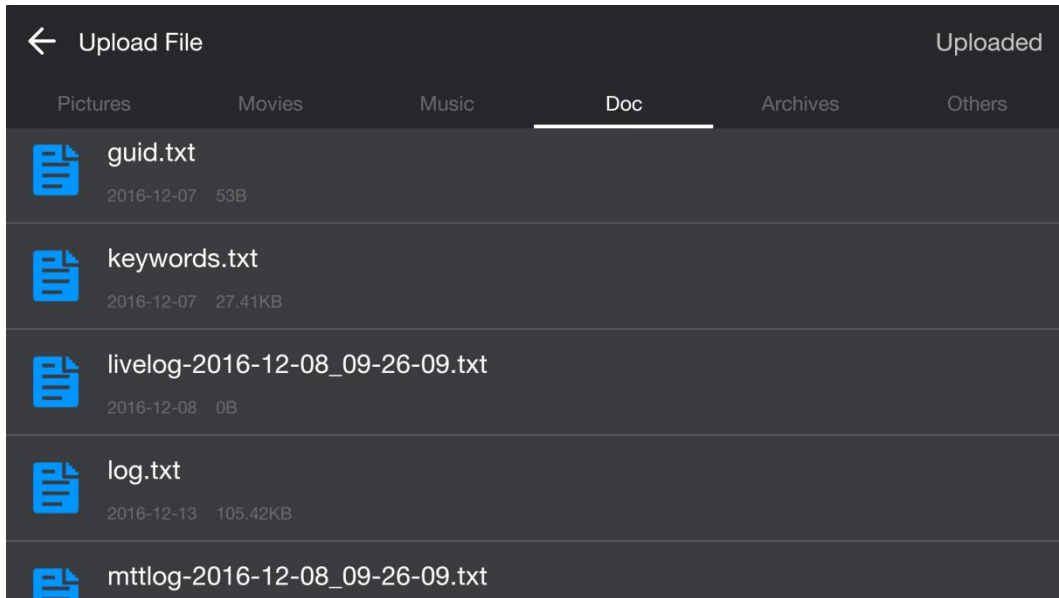
Figure 3-2-5-3 Upload document
