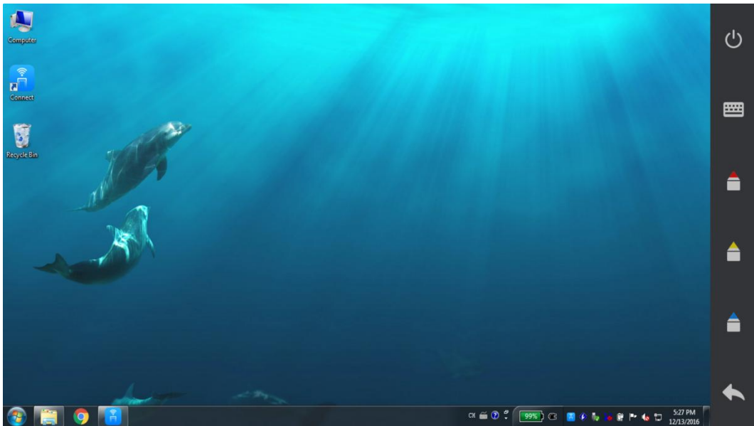
Figure 3-2-4-1 Remote desktop
