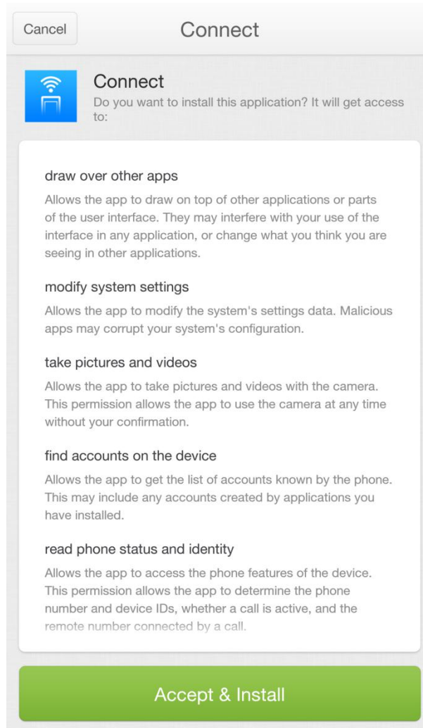
Figure 2-3-1 Installation interface
